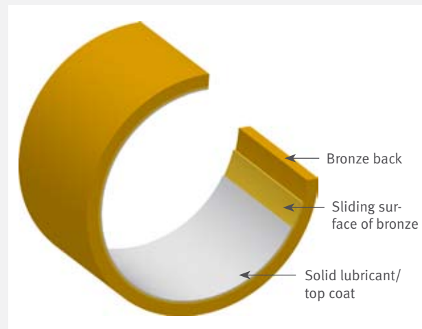
Layer system: bronze back / sliding surface of bronze / solid PTFE lubricant
